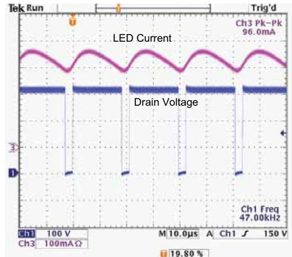
Steady State waveforms at 230VAC input and full load output
